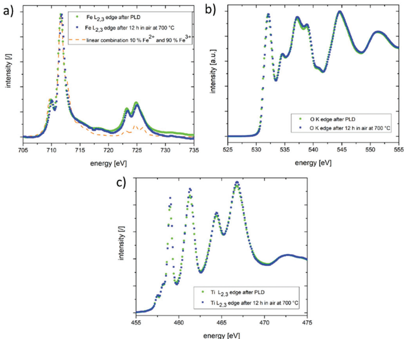
Figure 6. X-ray absorption measurements in fluorescence mode showing the a) Fe L 2,3 -edge, b) O K-edge, and c) Ti L 2,3 -edge of Fe-doped SrTiO 3 thin films deposited from a stoichiometric target with 2% Fe directly after the pulsed laser deposition (green dots) and after an additional annealing step at 700 °C in air for 12 h (blue squares). A linear combination of 10% Fe 2+ and 90% Fe 3+ (orange dashed line) matches the experimental data best.
